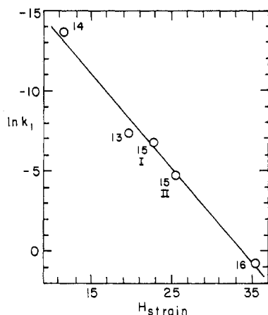
Figure 2. Correlation of strain energy with \ln k_1 for the aquation of \text{trans-Co}([13-16]\text{aneN}_4)\text{Cl}_2^+ , 25 °C, 0.1 M \text{HNO}_3 .
