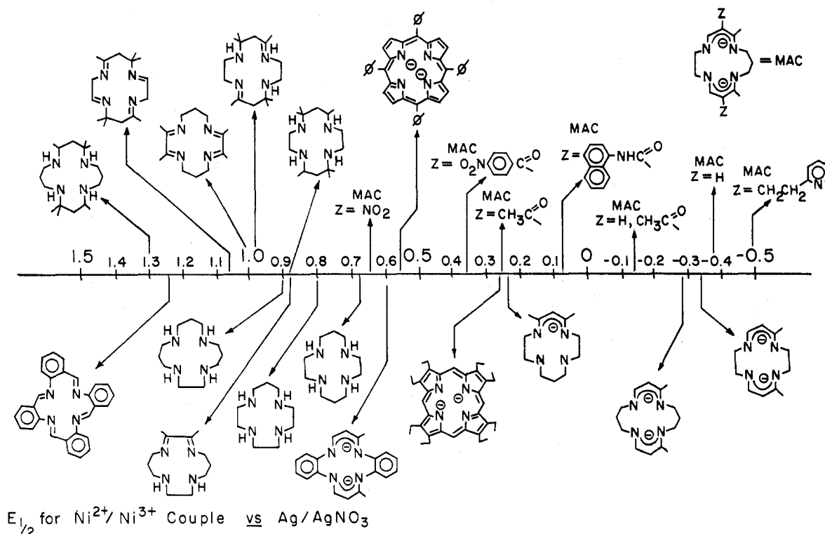
Figure 3. E_{1/2} for the Ni^{2+}/Ni^{3+} couple in tetraaza macrocyclic complexes vs. Ag/AgNO_3 , 0.1 M, reference electrode in CH_3CN . 59
